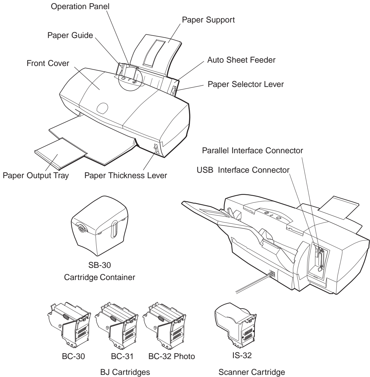
Figure 1-1 Printer Appearance
