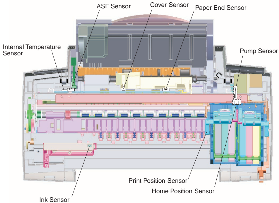
Figure 5-7 Sensor Positions
