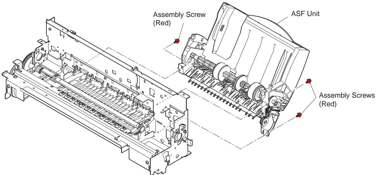
Figure 2-7 Removing the ASF Unit
