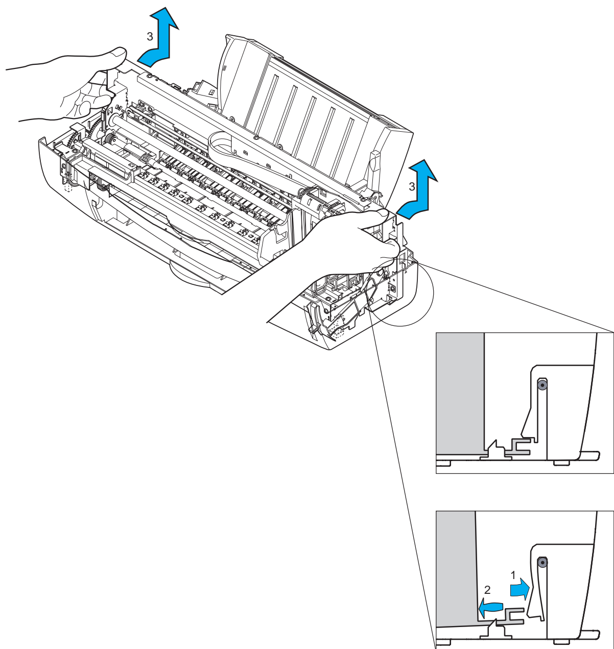
Figure 2-6 Removing the Printer Unit
