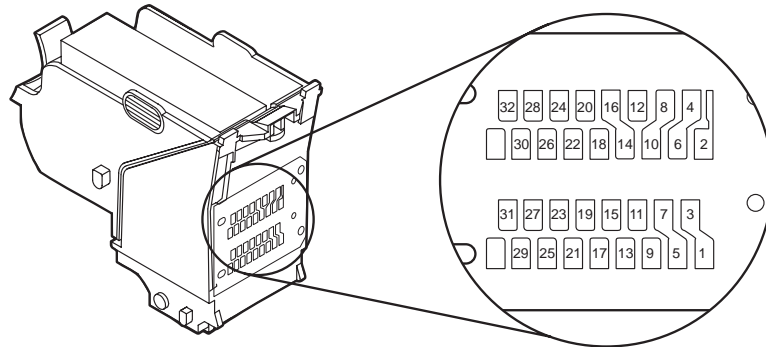
Figure 5-11 BJ Cartridge
