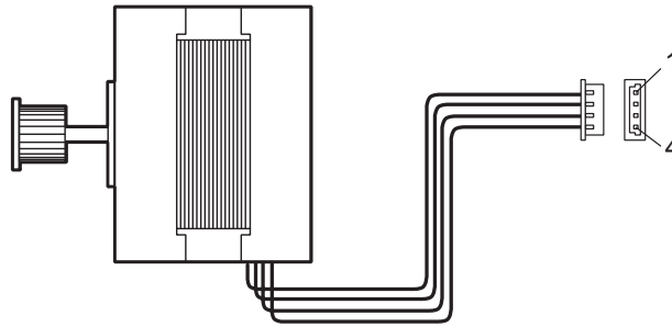
Figure 5-15 Carriage Motor
