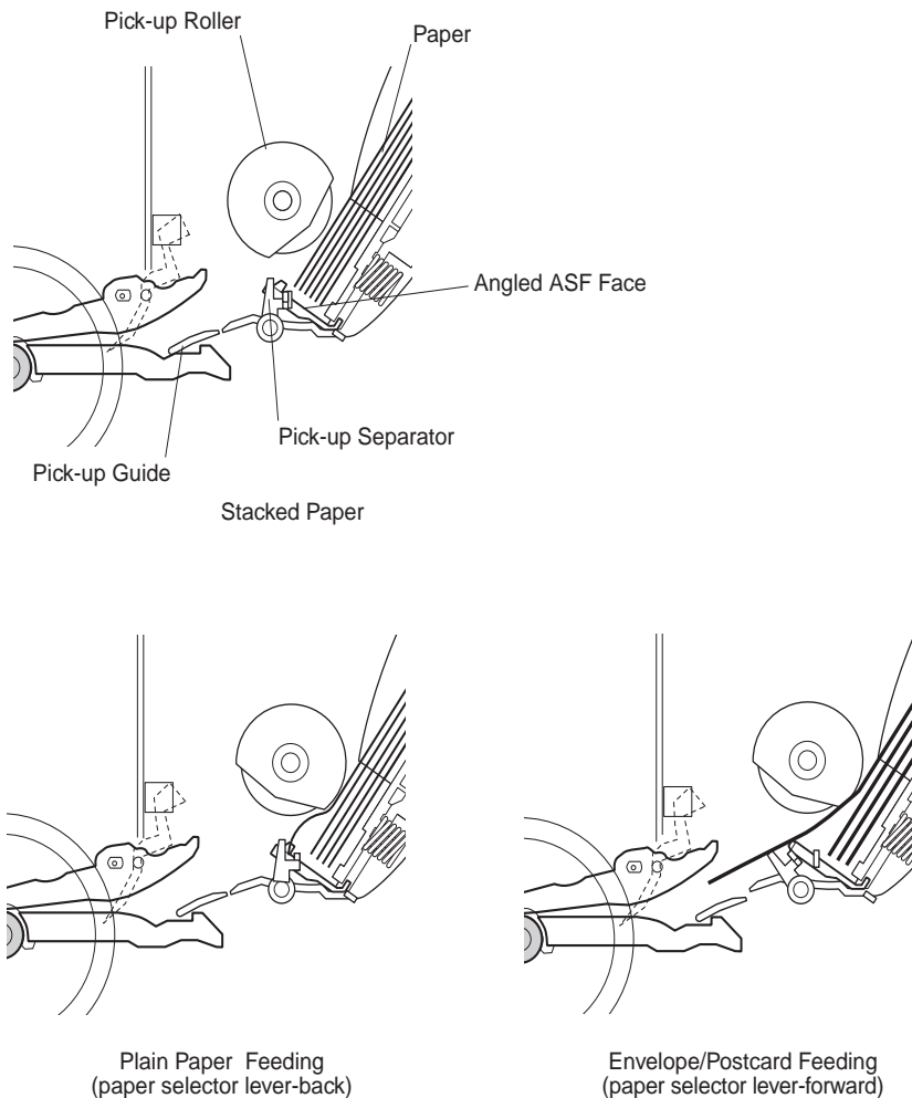
Figure 5-2 Paper Pick-up Unit
