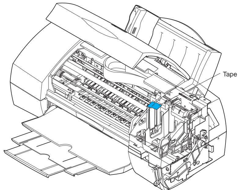
Figure 2-3 Capping Position
