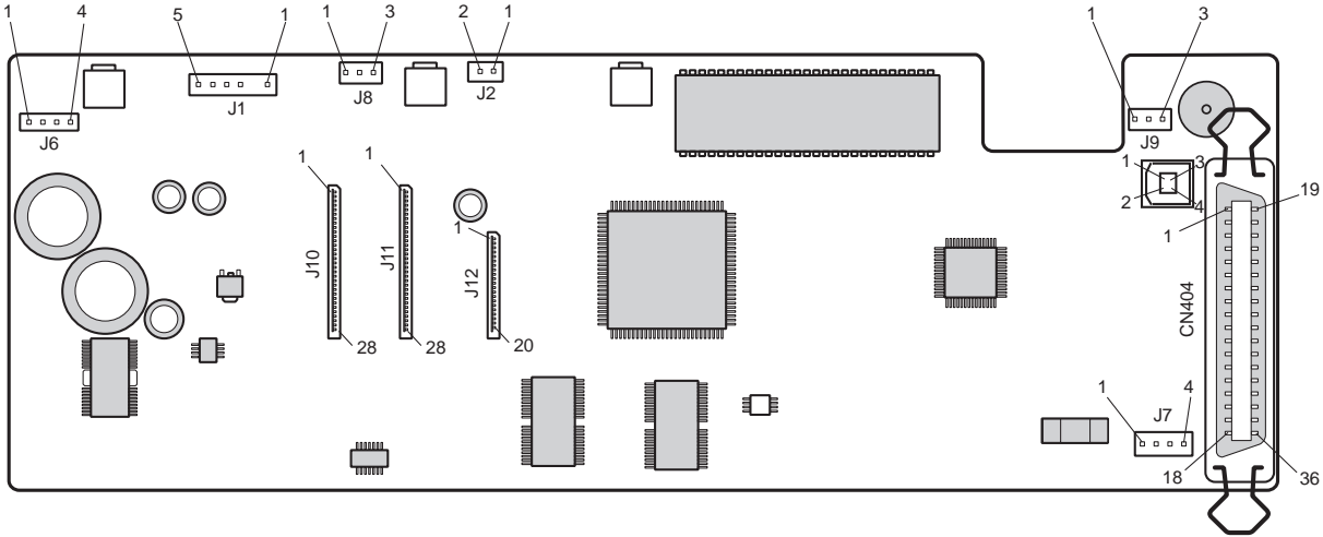
Figure 5-8 Control Board
