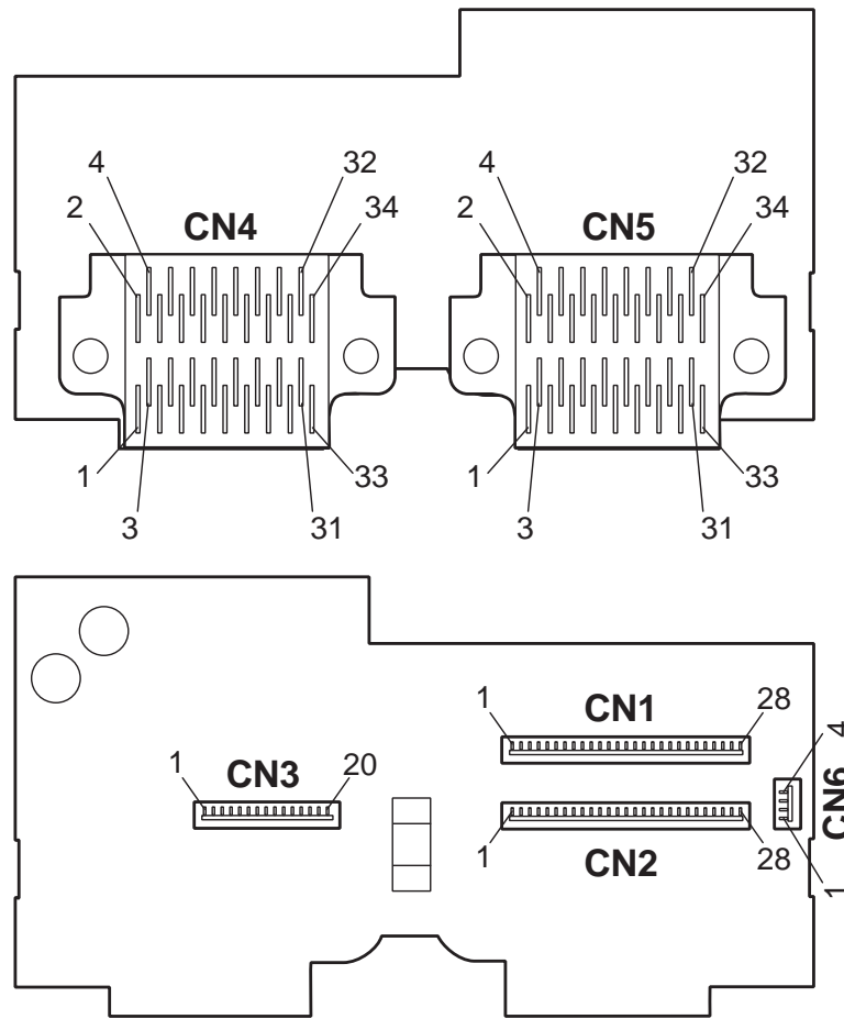
Figure 5-10 Carriage Board
