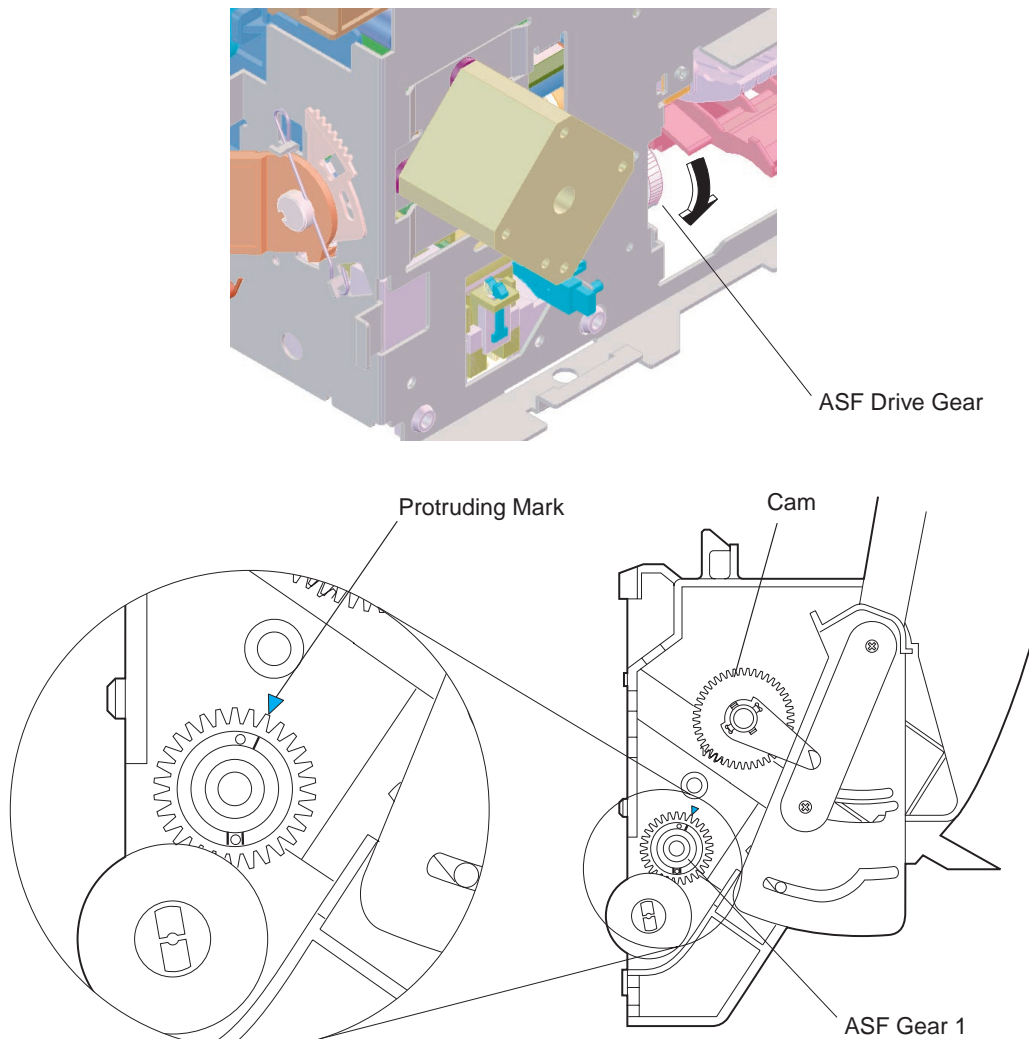
Figure 2-14 ASF Gear Position Adjustment 1
