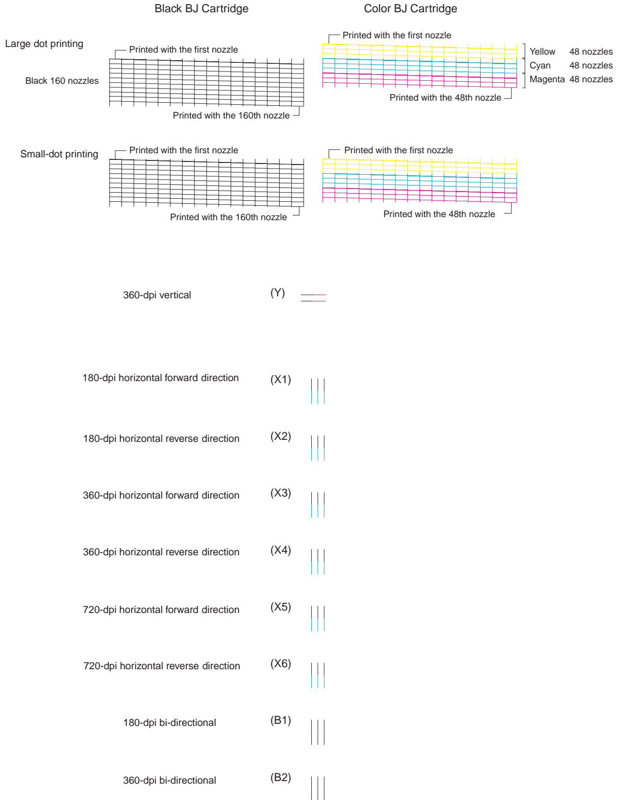
Figure 3-4 Nozzle Check Pattern Print (Sample for Black/Color Cartridge)
