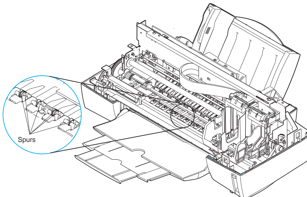
Figure 2-4 Spur Unit
