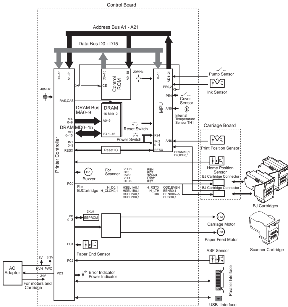
Figure 5-9 Block Diagram
