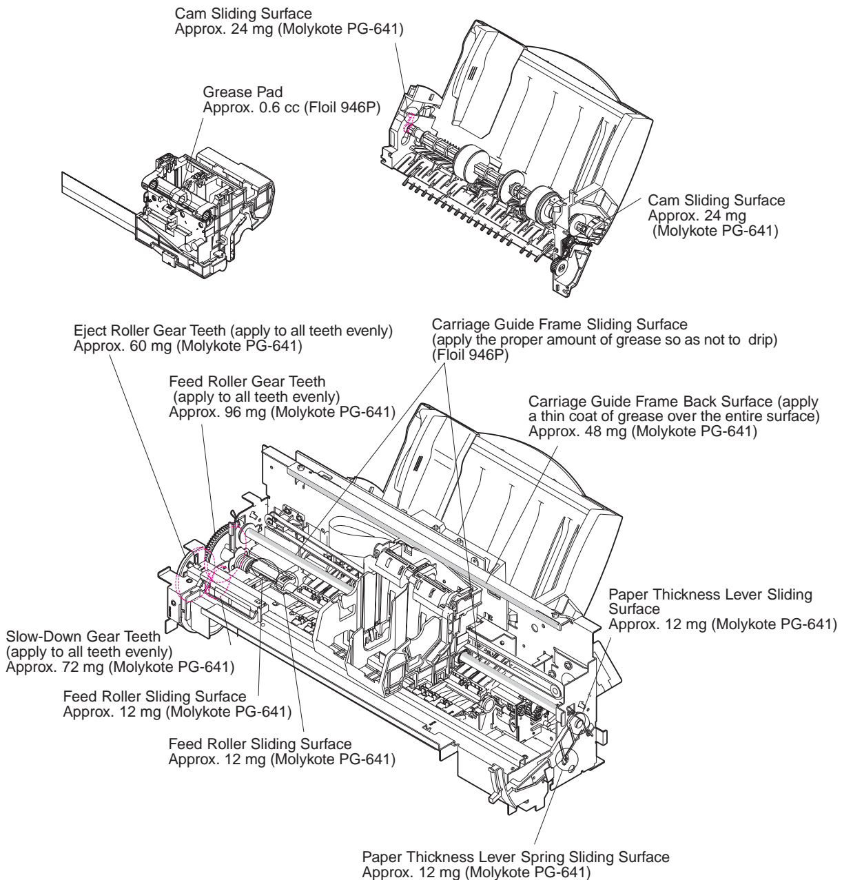
Figure 2-11 Grease Points
