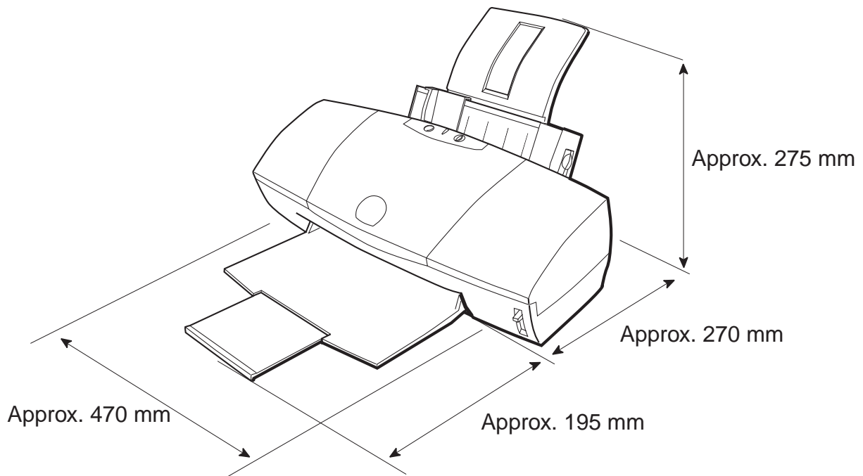
Figure 5-21 Printer Dimensions
