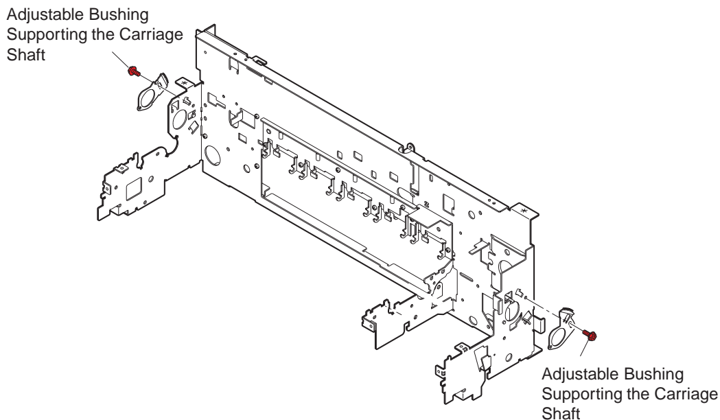
Figure 2-8 Adjustable Bushings Supporting the Carriage Shaft
