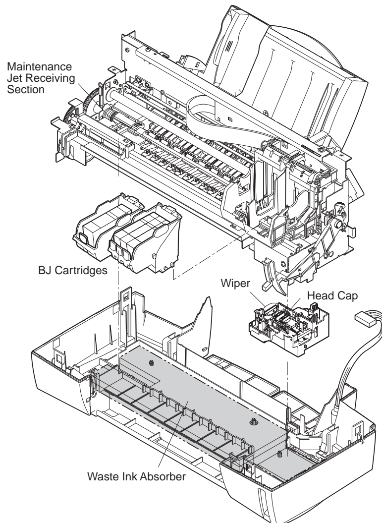
Figure 2-1 Ink Paths
