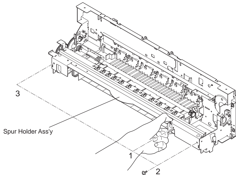
Figure 2-10 Spur Holder Ass'y Installation
