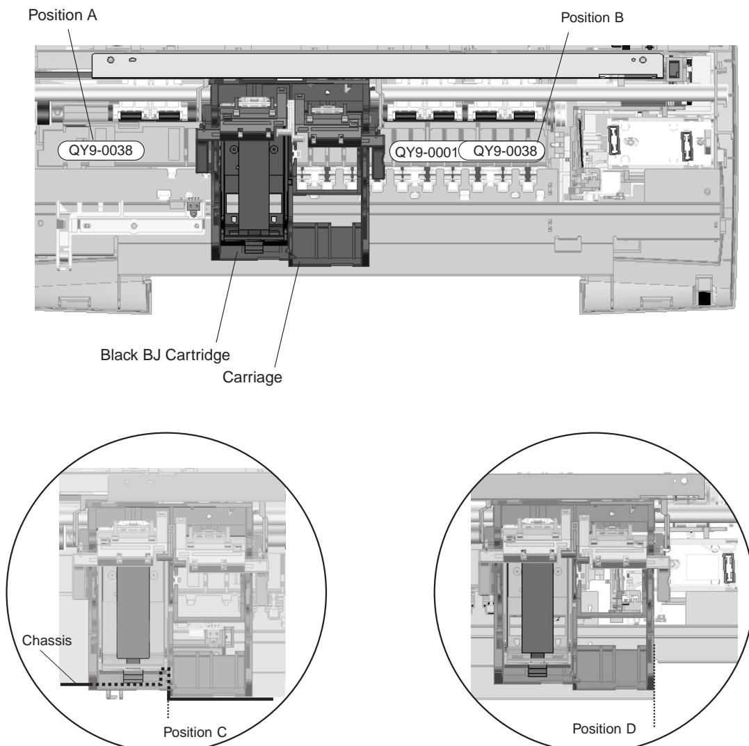
Figure 2-17 Head Gap Adjustment 2
