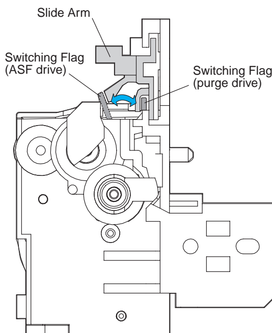
Figure 5-6 Operation of the Drive Switching Unit
