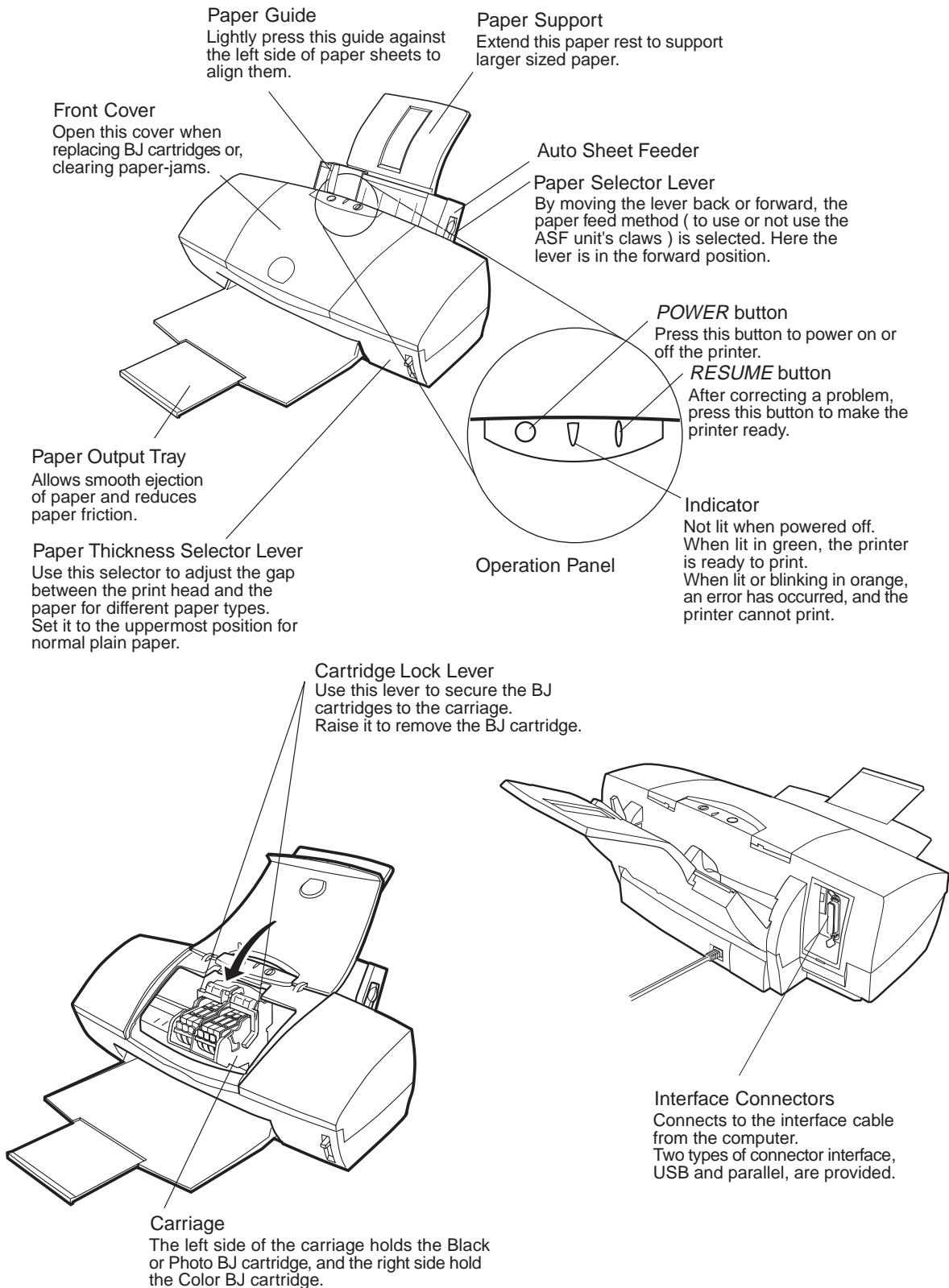
Figure 1-5 Names of Parts and Their Functions
