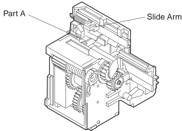
Figure 5-5 Drive Switching Unit
