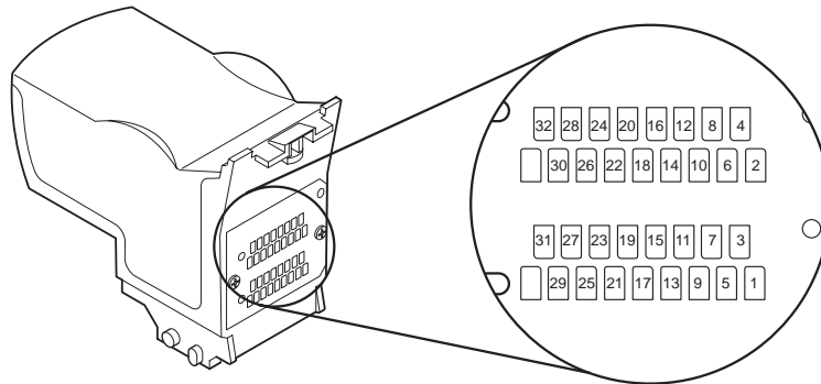
Figure 5-12 Scanner Cartridge
