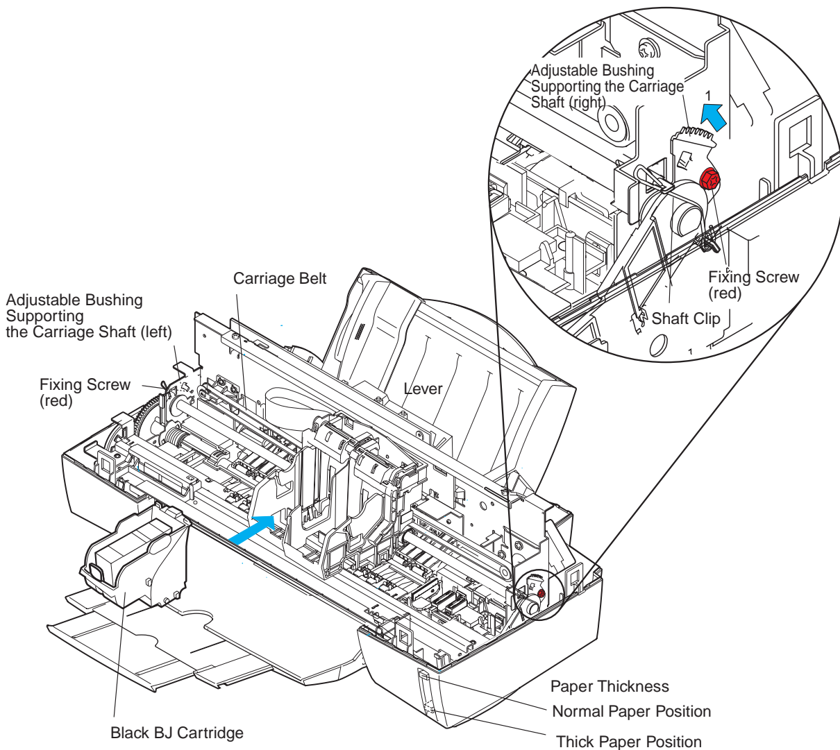
Figure 2-16 Head Gap Adjustment 1
