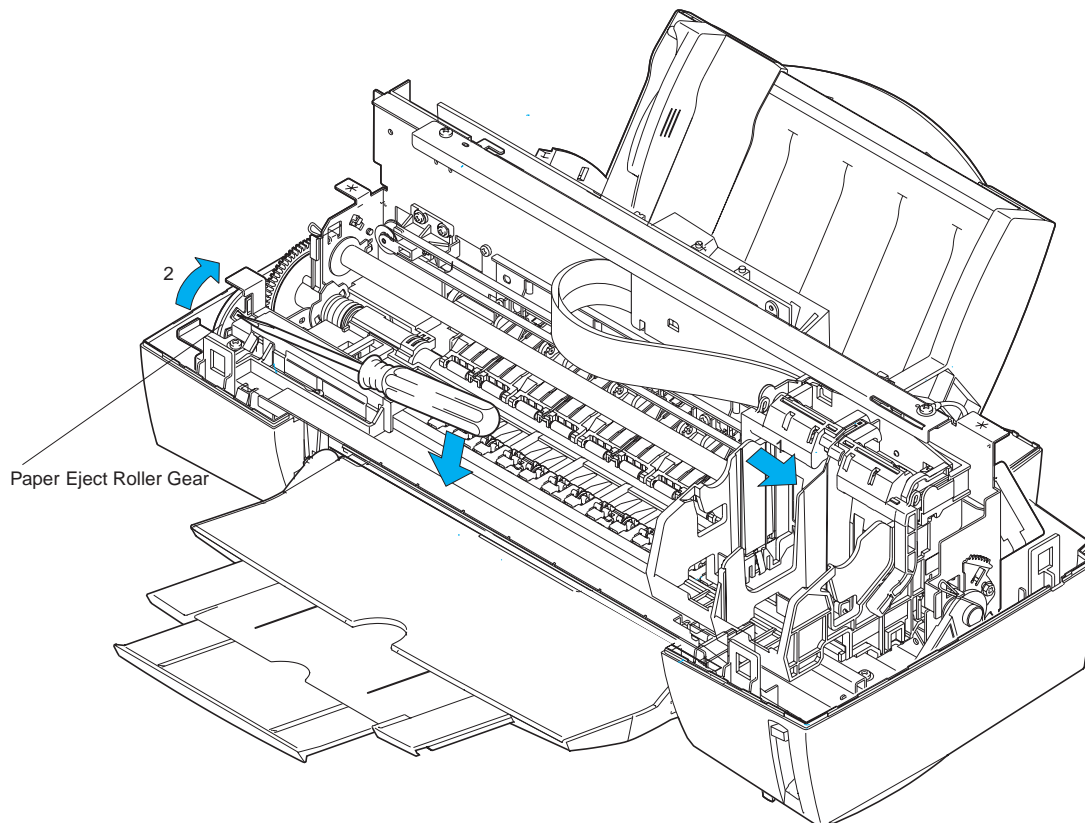
Figure 2-5 Unlocking the Carriage
