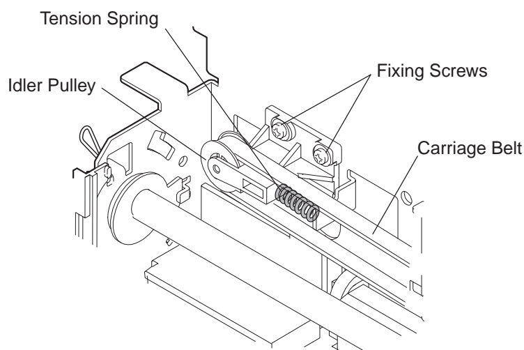
Figure 2-13 Carriage Belt Tension Adjustment
