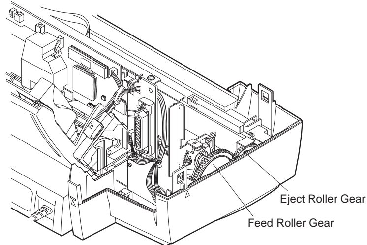
Figure 2-9 Paper Feed Gears
