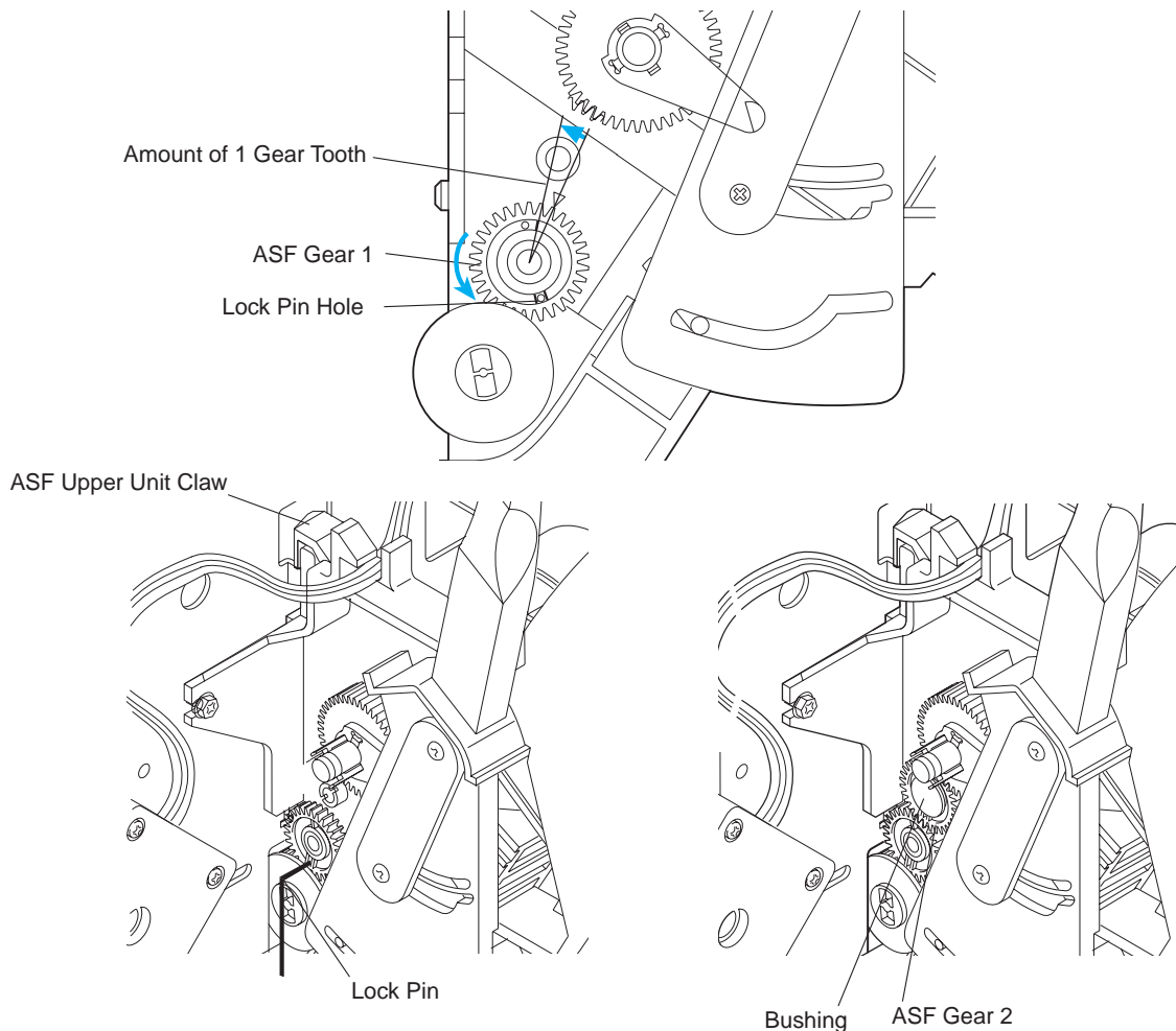
Figure 2-15 ASF Gear Position Adjustment 2
