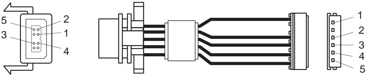
Figure 5-14 DC Power Supply Cable
